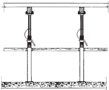
Single-Post Shores with Lateral Bracing
