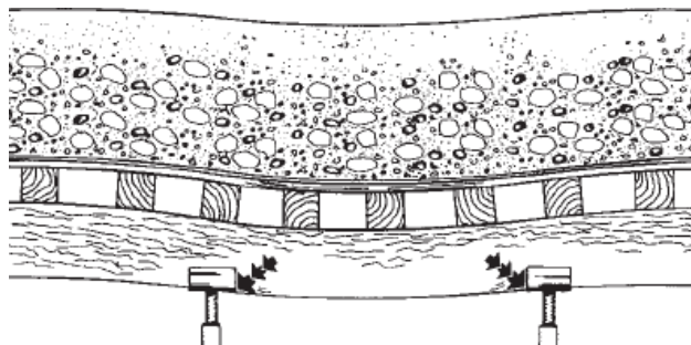
Deflection of Stringers Between Supports
