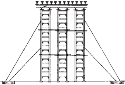
Typical Shoring Tower with Stringers, Adjustable Base Plates, and U-Heads
