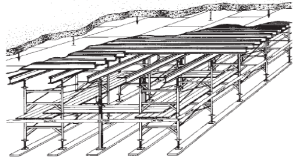
Two Rows of Shoring Frames
