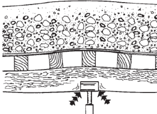
Deflection of Stringers Between Supports
