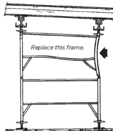
Frame Bent out of Shape
